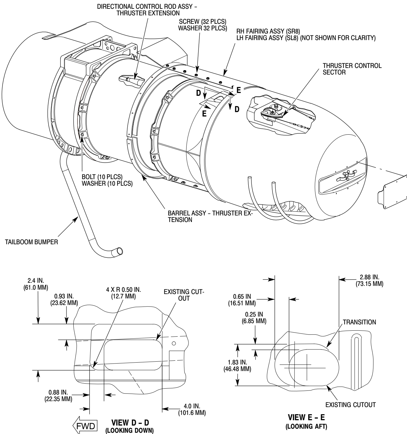
Figure 1. Thruster Modification
