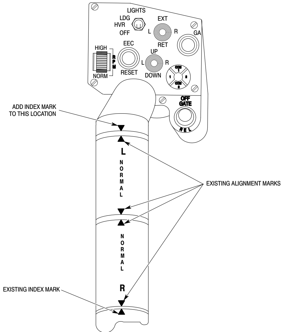
Figure 1. Application of Index Mark to Collective Control Module
