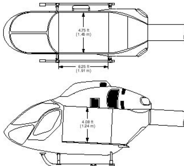
Figure 35. Main Cabin Dimensions
